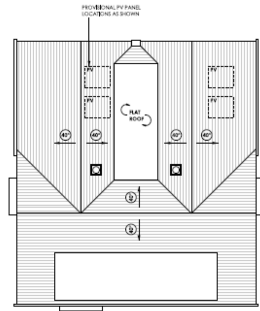
ROOF PLAN
